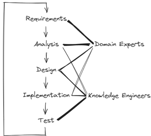
FIGURE 14.1: Semantic web design workflow.
