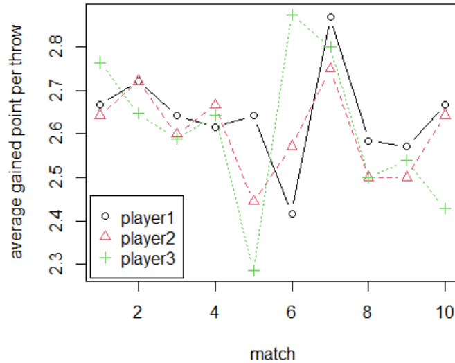
FIGURE 7.5: Plot of average point gained per throw attempt for the 3 players in 10 matches.
