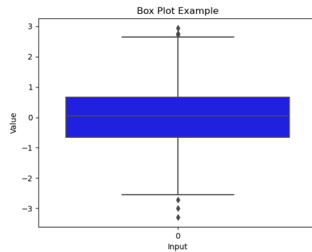
FIGURE 9.4: Box plot using Seaborn. The box gives IQR. The bars below and above the box give Q_1 - 1.5 \times \text{IQR} and Q_3 + 1.5 \times \text{IQR} , respectively. The dots are outliers.
