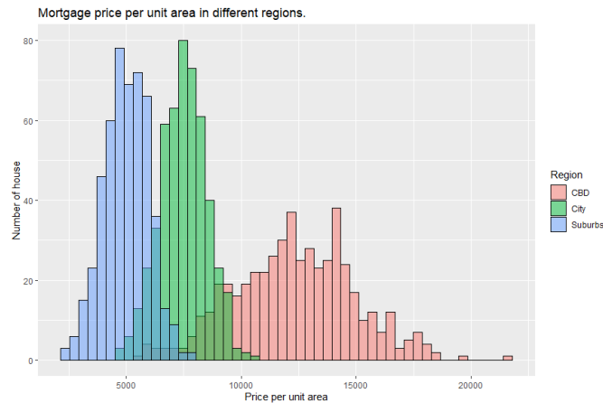
FIGURE 7.12: An example of histogram plot of house price per unit area in different regions in a single plot.
