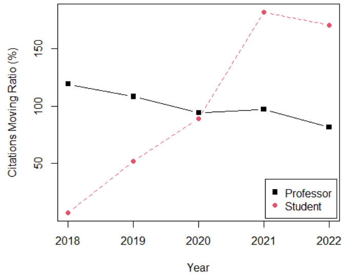
FIGURE 7.3: A demonstration of using matplot to plot trends.
