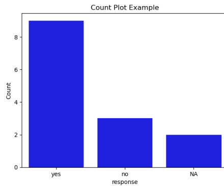
FIGURE 9.3: Count plot using Seaborn.
