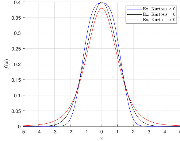
FIGURE 1.3: Demonstration of PDF with different excess kurtosis.
