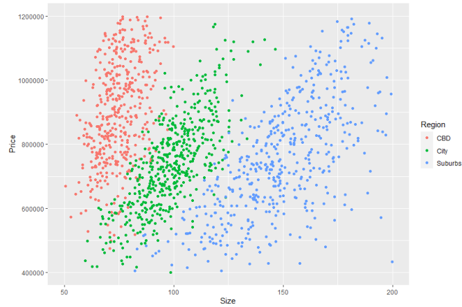
FIGURE 7.15: Add coordinates layer using xlim() and ylim() .
