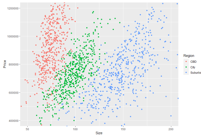
FIGURE 7.16: Add coordinates layer using coord_cartesian() .
