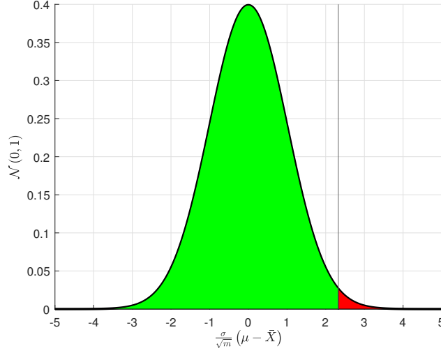
FIGURE 5.1: Distribution of scaled estimation error, where the green zone corresponds with the probability of 0.99 and the red zone, 0.01.
