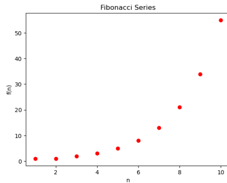
FIGURE 9.1: Plot Fibonacci series as scatter plot.
