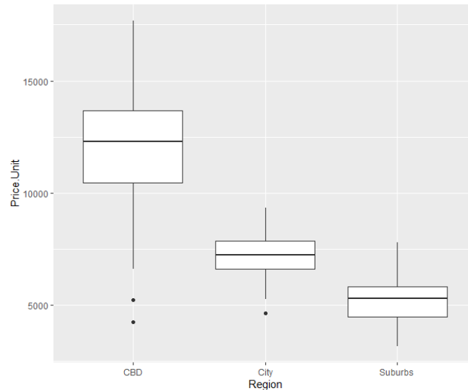
FIGURE 7.8: A second demonstration of qplot on mortgage price data frame.
