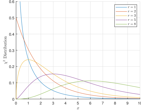
FIGURE 2.6: The \chi^2 Distribution.
