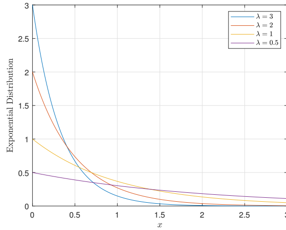
FIGURE 2.3: Exponential distributions with different \lambda .
