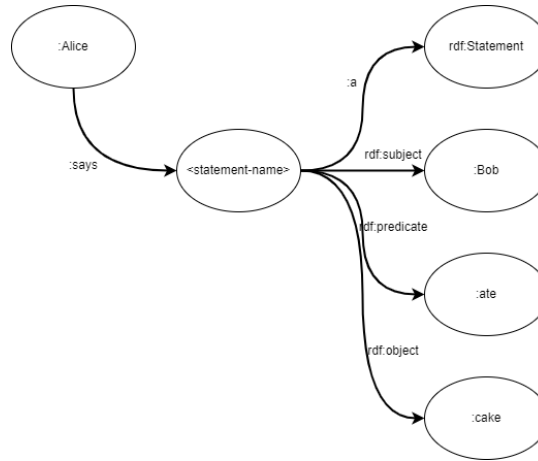
FIGURE 12.7: An example of RDF reification.
