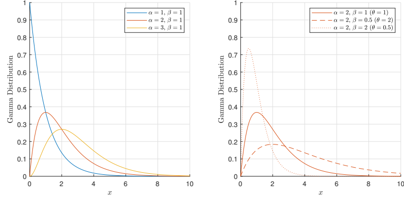
FIGURE 2.5: Gamma Distribution.
