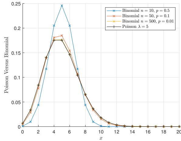
FIGURE 2.2: Poisson distribution approximation using binomial distribution.
