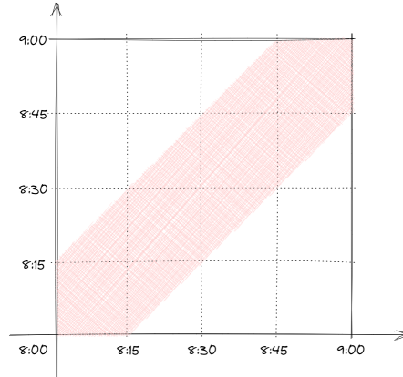
FIGURE 1.1: Sample space of two people arriving at the park from 8:00 AM to 9:00 AM.
