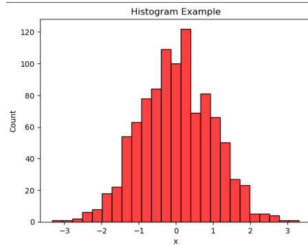
FIGURE 9.2: Histogram plot using Seaborn.
