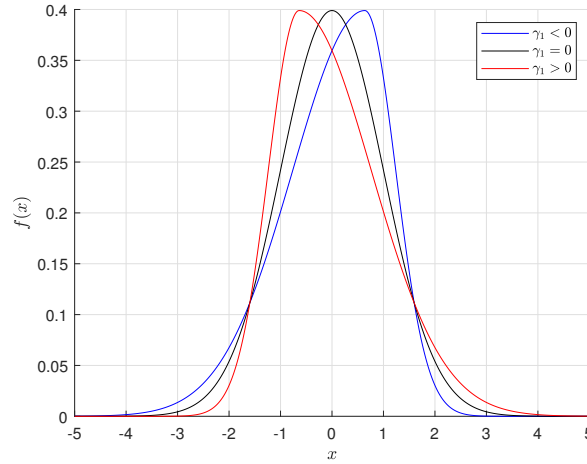
FIGURE 1.2: Demonstration of PDF with different skewness.
