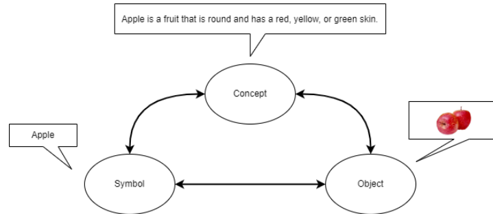
FIGURE 12.1: Semiotic triangle of Apple.
