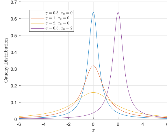
FIGURE 2.4: Cauchy Distribution.
